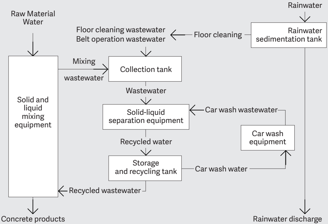
RMC Plant Water Balance Diagram
